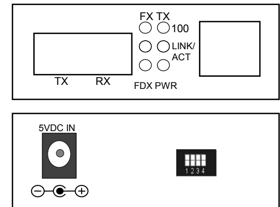
Fig. 1 Fast Ethernet Switching Converter Front & Rear Panel
