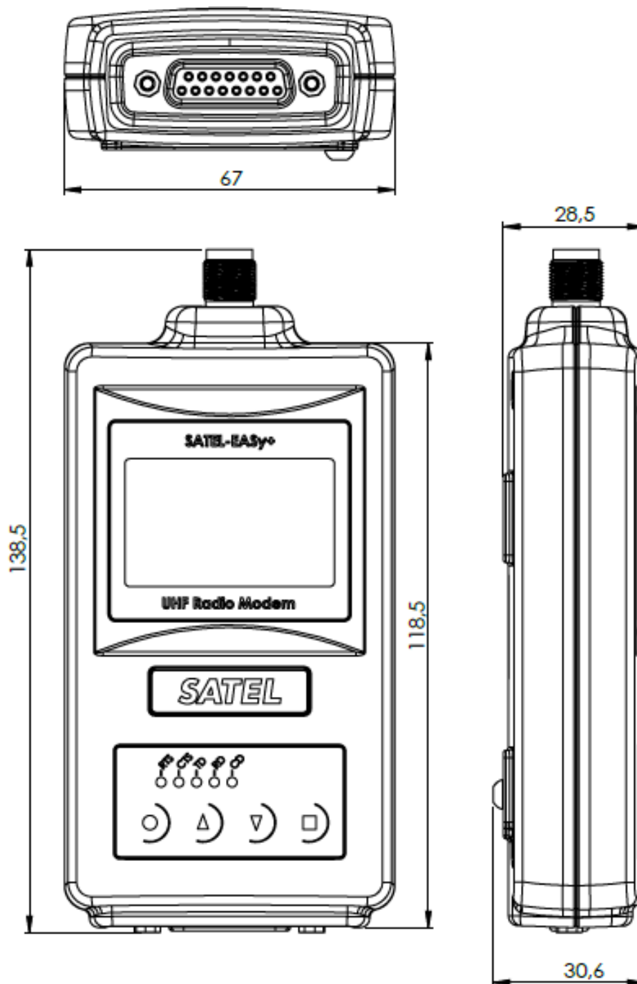
Figure 1.1 SATEL-EASy+ (variant 1) mechanical dimensions
