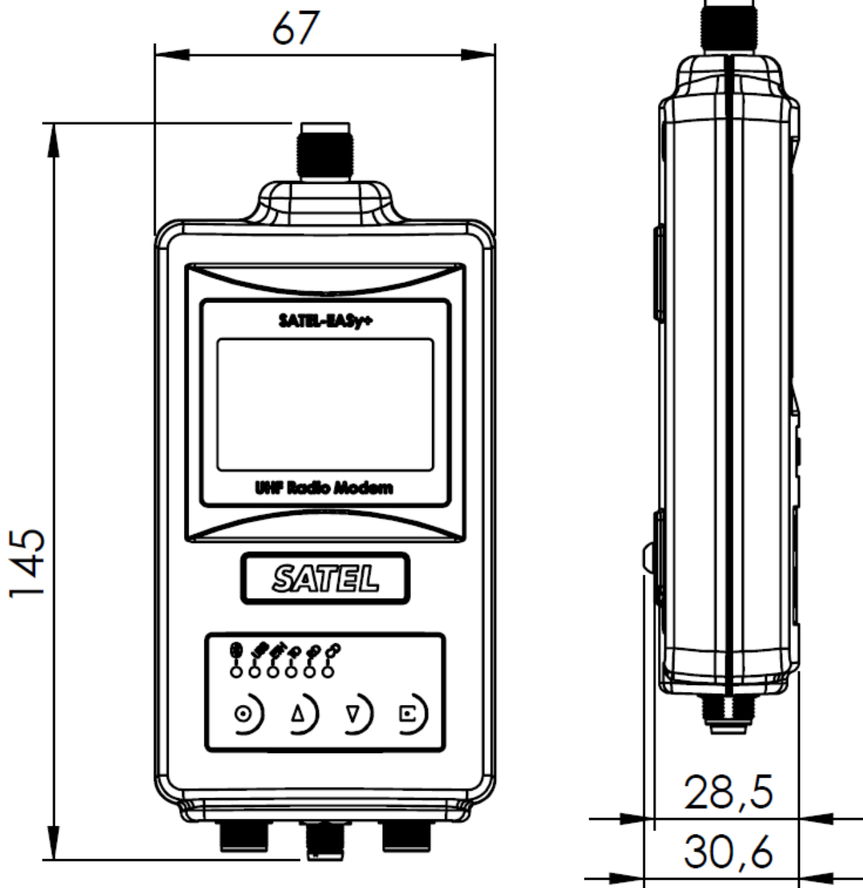
Figure 1.2 SATEL-EASy+ (variant 2) mechanical dimensions
