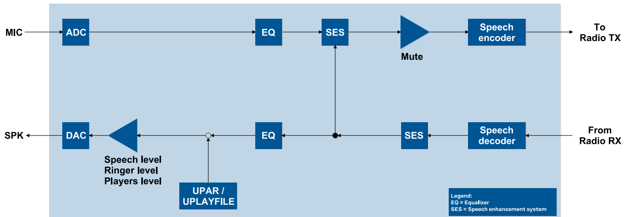
Figure 23: SARA-G4 series audio paths
