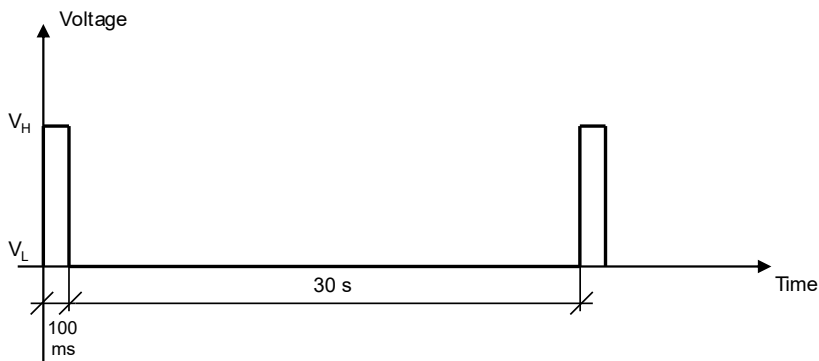
Figure 7: GPIO pin progress for registered home network NB1 / NB2
