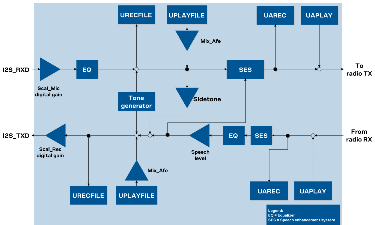
Figure 16: LARA-R211 audio paths
