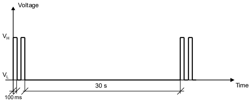
Figure 10: GPIO pin progress for registered roaming NB1 / NB2
